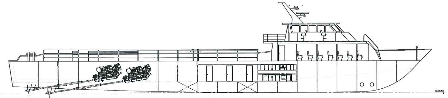
INBOARD PROFILE
