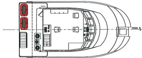
UPPER DECK PLAN
